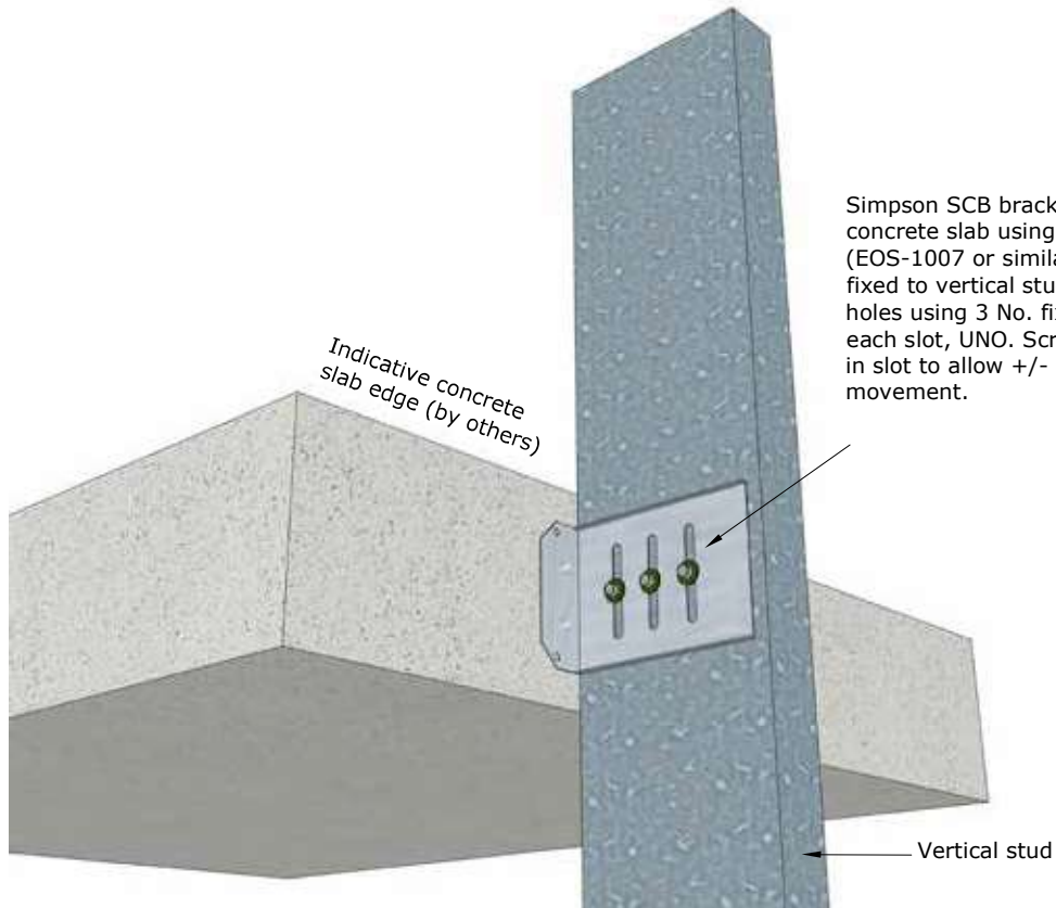
TYPICAL OVERSAIL STUD FIXING
