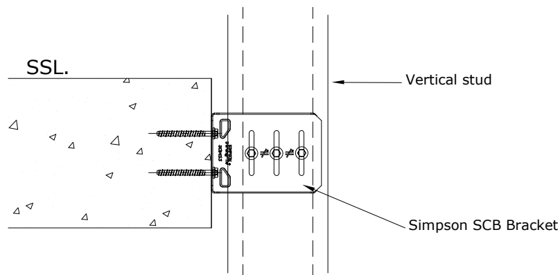
TYPICAL SECTION
